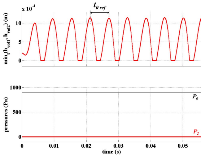
FIG. 11. (Color online) Two-mass simulations of \min(h_{\text{vof}_1}(t), h_{\text{vof}_2}(t)) and P_2(t) as a function of time. Configuration of reference with h_{\text{venf}}(t) = h_{\text{ventricle}} , P_0 = 900 Pa, 1/t_{0\text{ref}} = 173 Hz (mean value). Input (resp. output) data are displayed in thin solid (resp. thick dotted) line.
