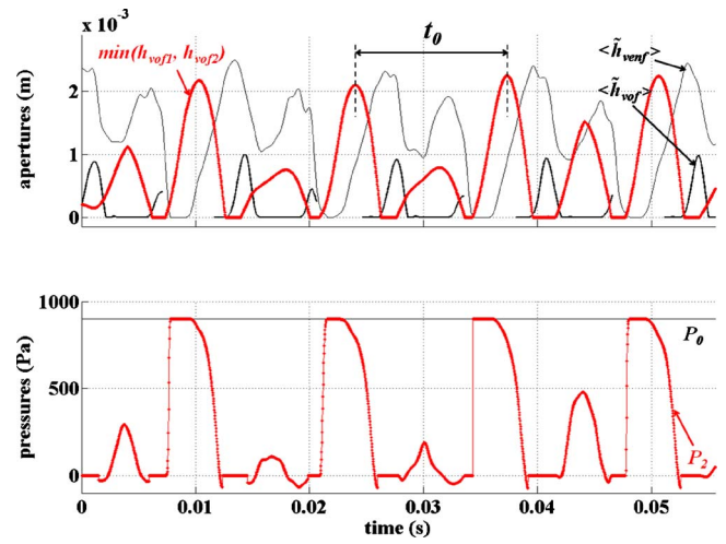
FIG. 12. (Color online) Two-mass simulations of \min(h_{\text{vof}_1}(t), h_{\text{vof}_2}(t)) and P_2(t) as a function of time. h_{\text{venf}}(t) = \langle \tilde{h}_{\text{venf}} \rangle(t) , P_0 = 900 Pa, 1/t_0 = 74 Hz (mean value). Input (resp. output) data are displayed in thin solid (resp. thick dotted) line.
